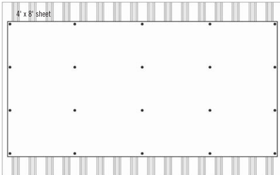
Figure B Top Side Drill Screw Pattern
