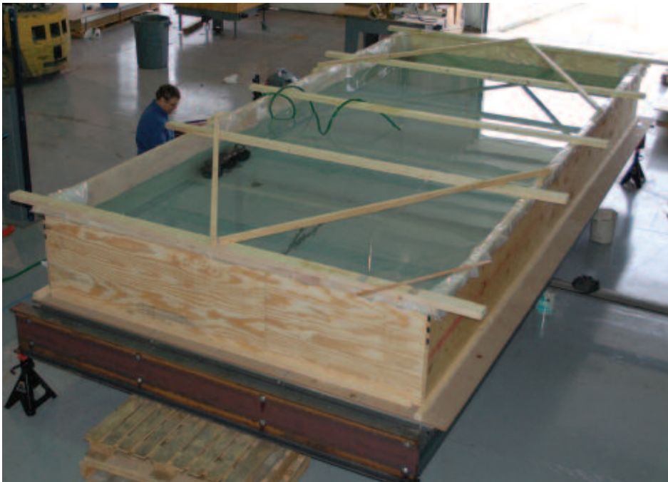
Cornerstone Specialty Wood Products recreates a uniform loading condition on a large platform.
