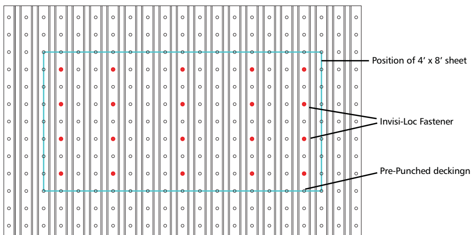
Figure A Invisi-LOC ® Underside Fastening System
