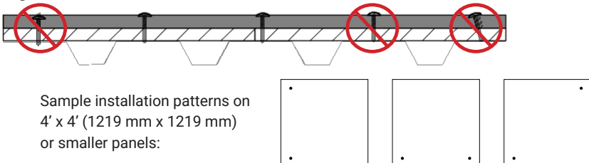
Figure H. ESD Screw Installation - Cross Section - Screws must be flush with deck surface!
